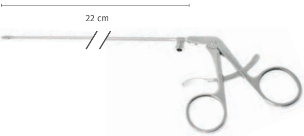
Portaguja para laringe con canal de irrigación, con trinquete, eje cónico (2.0 - 3.0 mm), 22 cm Laryngeal needle-holder with irrigation channel, with ratchet, conical shaft (2.0 - 3.0 mm), 22 cm 50-650-23
